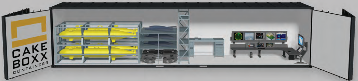
Side opening container - safe, secure, and efficient loading configurations for UUV, UAV, UGV, plus command and control equipment
